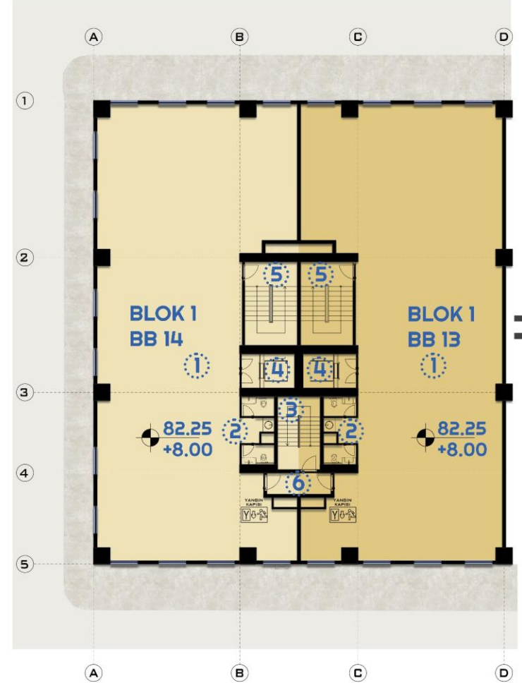
BİRİNCİ KAT KİSMİ PLAN
