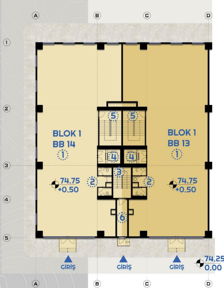
ZEMİN KAT KİSMİ PLAN
